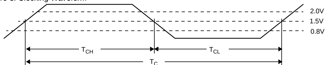
Figure 3. Clocking Waveform
