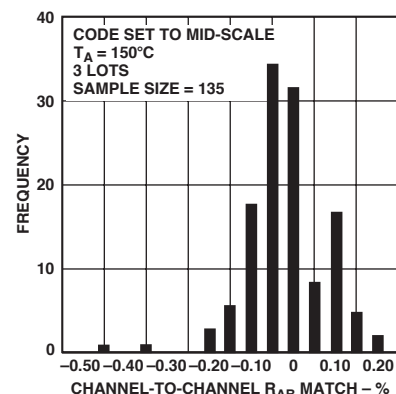
TPC 29. Channel-to-Channel Resistance Matching (AD5262)
