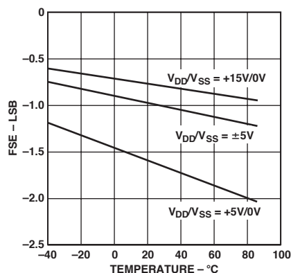
TPC 10. Full-Scale Error
