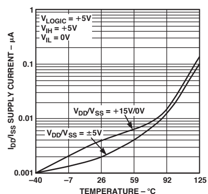
TPC 12. Supply Current vs. Temperature
