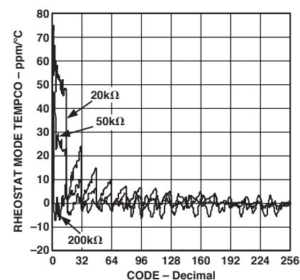
TPC 15. Rheostat Mode Tempco \Delta R_{WB}/\Delta T vs. Code
