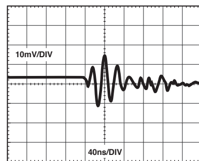
TPC 26. Digital Feedthrough vs. Time
