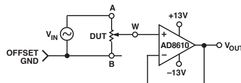
Test Circuit 5. Gain vs. Frequency
