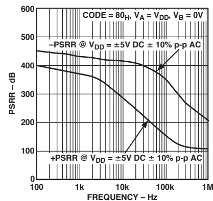
TPC 23. PSRR vs. Frequency
