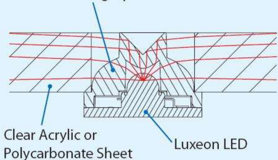
Side-Emitting Optic
