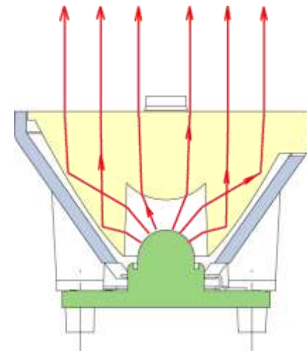
Diagram showing light ray paths through a TIR optic
