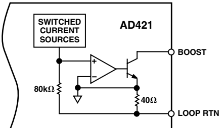
Figure 4. Current Amplifier
