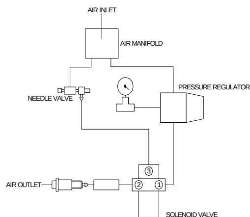
PNEUMATIC DIAGRAM
