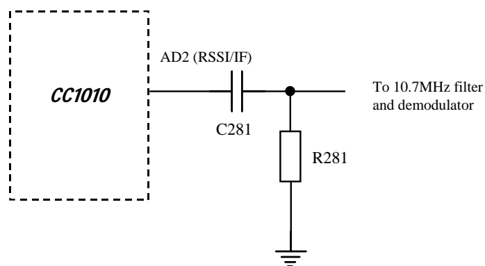
Figure 43. IF Output
