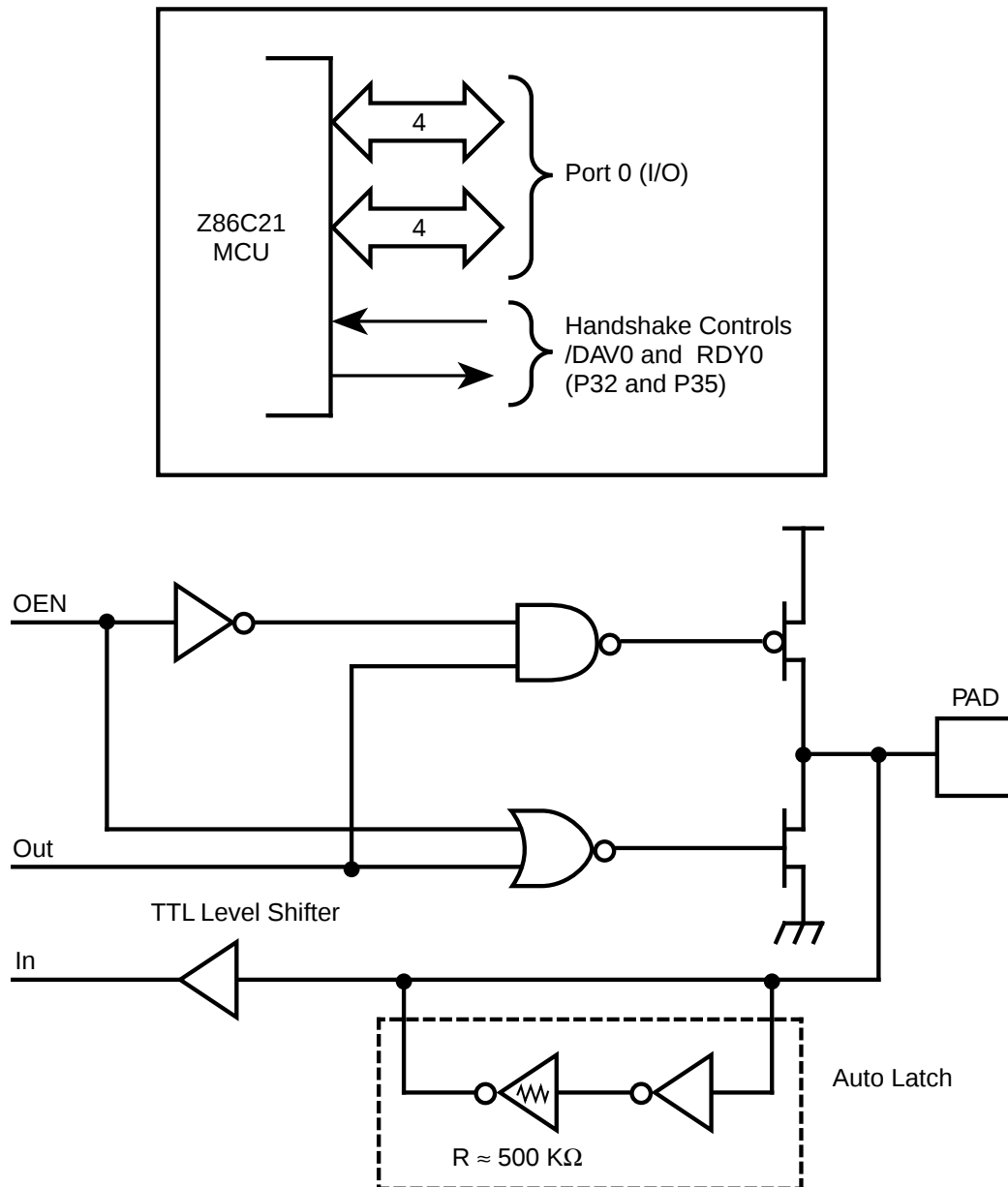
Figure 5. Port 0 Configuration
