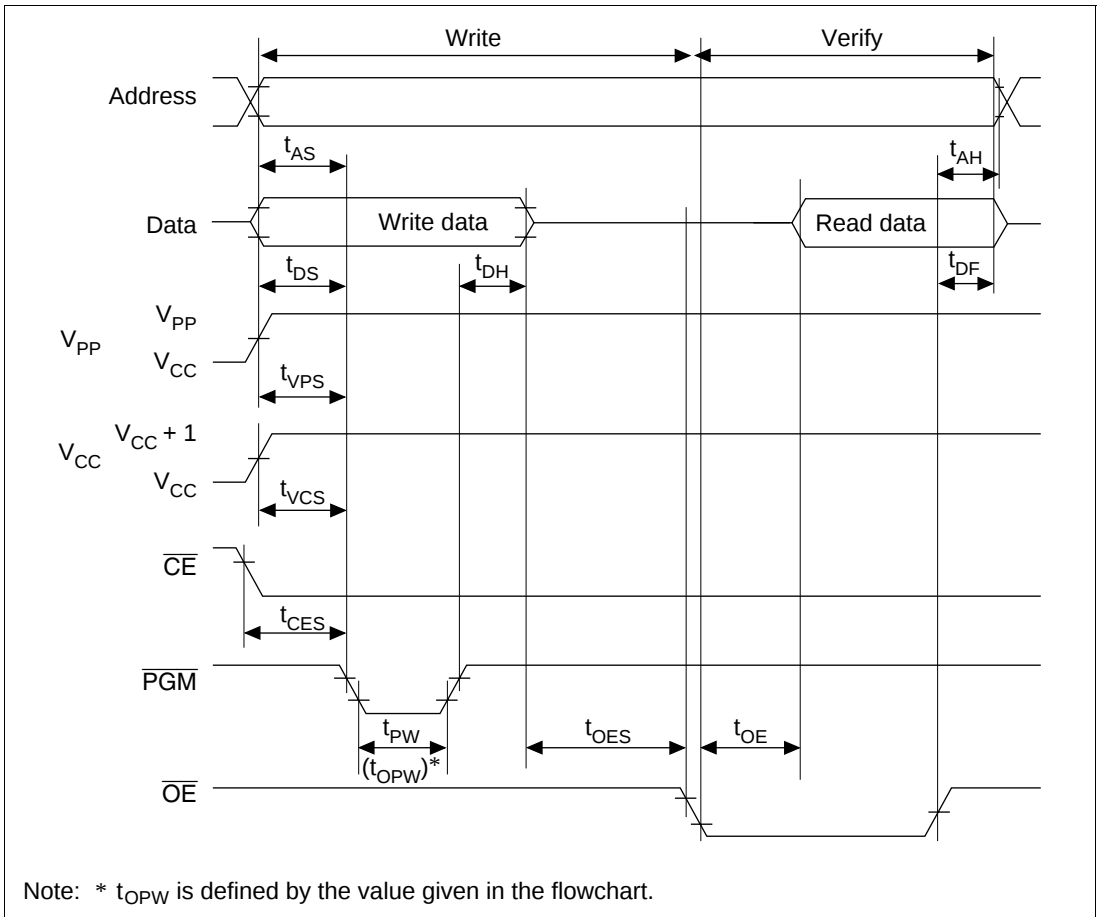
Figure 17.5 Write/Verify Timing
