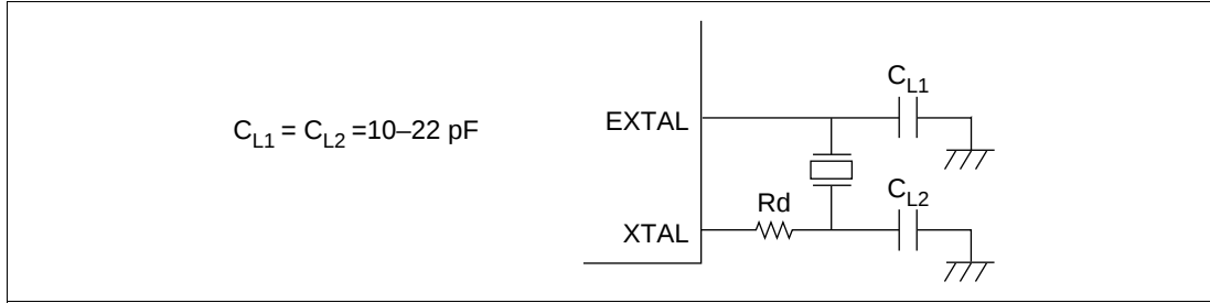
Figure 7.2 Connection of Crystal Resonator (Example)
