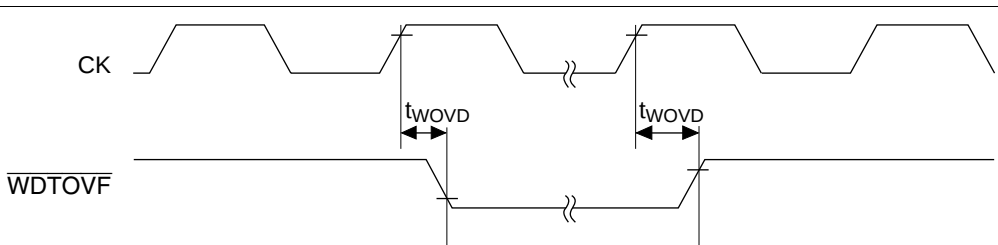
Figure 20.39 Watchdog Timer Output Timing
