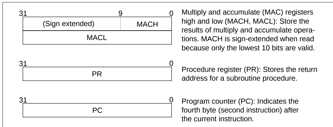
Figure 2.3 System Registers
