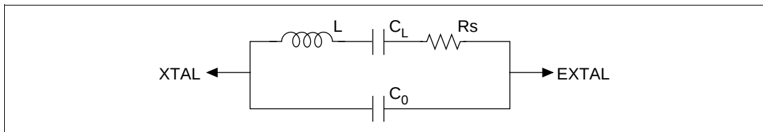
Figure 7.3 Crystal Resonator Equivalent Circuit
