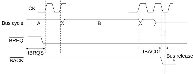
Figure 8.43 When \overline{\text{BREQ}} is Input without Satisfying tBRQS
