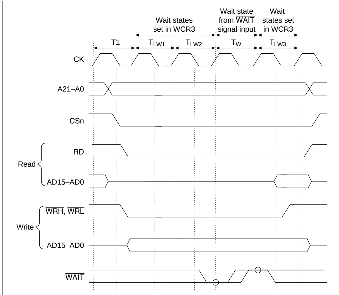
Figure 8.14 Wait State Timing for External Memory Space Access (1 State Plus Long Wait State (When Set to Insert 3 States) Plus Wait States from \overline{WAIT} Signal)
