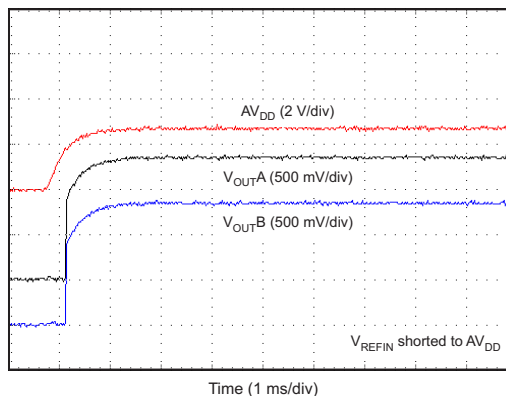
Figure 86. Power-On Glitch Reset to Mid-Scale
