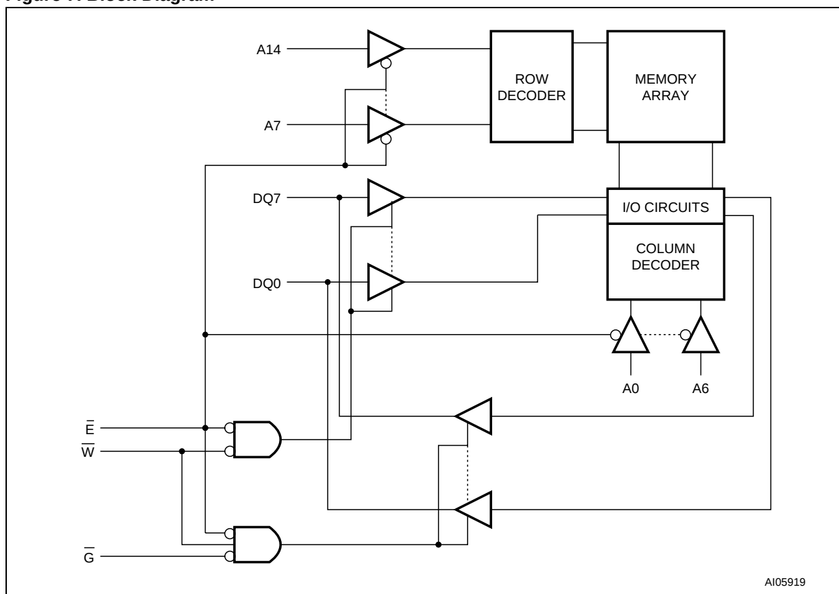
Figure 7. Block Diagram
