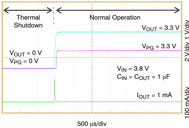
Figure 37. Recovery from Thermal Shutdown NCP752A, V_{\text{OUT}} = 3.3\text{ V}
