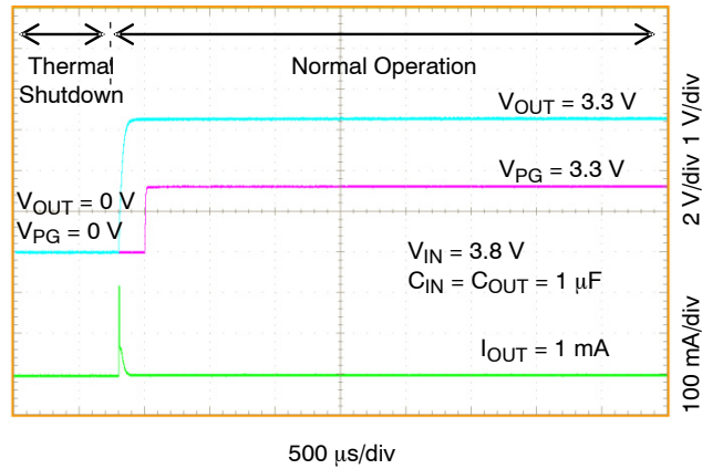
Figure 38. Recovery from Thermal Shutdown NCP752B, V_{\text{OUT}} = 3.3\text{ V}
