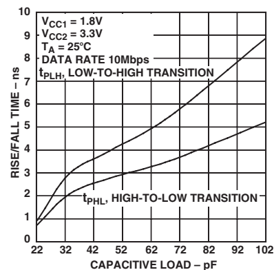
TPC 12. Rise/Fall Time vs. Capacitive Load, A1/A2-Y1
