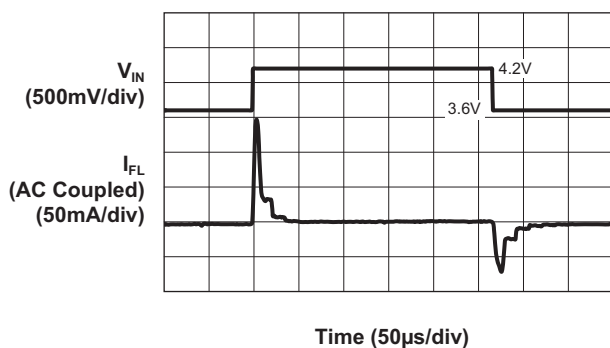
Movie Mode Line Transient (I_{\text{FLOUT}} = 206\text{mA}; V_{\text{IN}} = 4.2\text{V to } 3.6\text{V})
