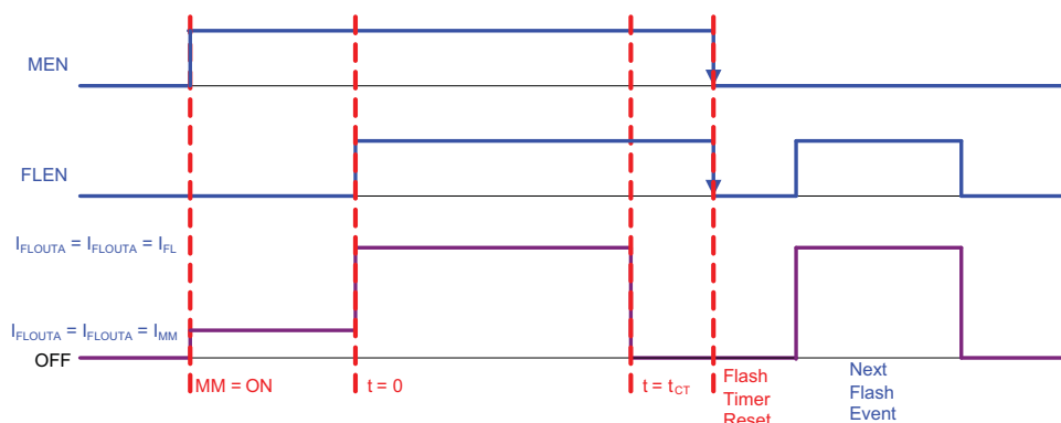
Figure 5: Diagram of Movie Mode Followed by Flash Mode
