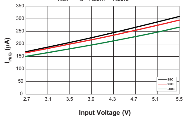
Quiescent Current vs. Input Voltage (V_{FLEN} = V_{IN}; I_{FLOUTA} = I_{FLOUTB} = 0mA)
