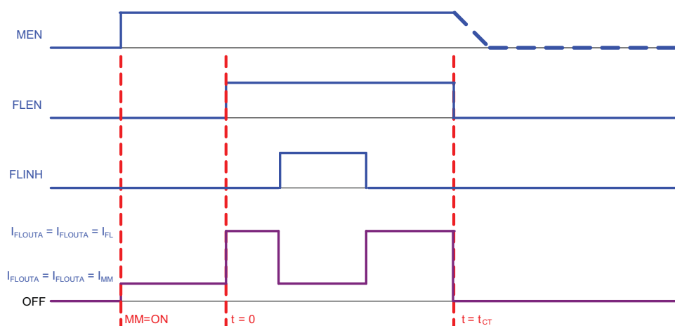
Figure 6: Diagram of Movie Mode Followed By Flash Mode
