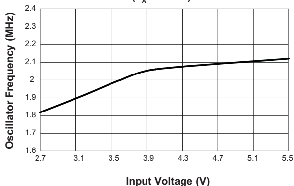
Oscillator Frequency vs. Input Voltage (T_A = 25^\circ\text{C})
