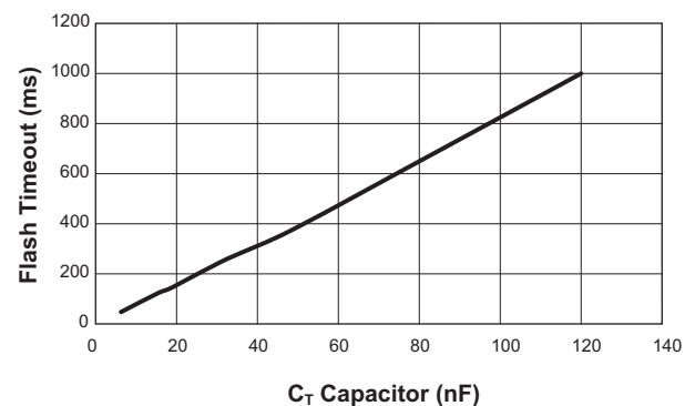
Figure 7: Flash Safety Timeout vs. Timer Capacitor.
