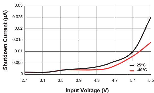
Shutdown Current vs. Input Voltage (V_{MEN} = V_{FLEN} = V_{FLINH} = 0V)
