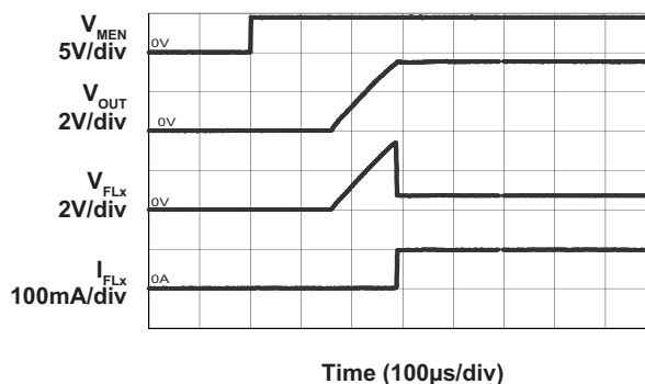
Movie Mode Turn On Characteristic
