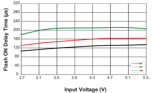
Flash ON Delay Time vs. Input Voltage (I_{FLOUTA} = I_{FLOUTB} = 750mA; C_{OUT} = 2.2\mu F; L = 1\mu H)
