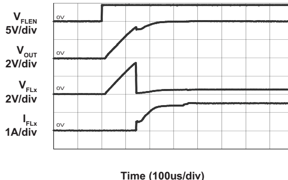
Flash Turn On Characteristic (I_{\text{FLOUTA}} = I_{\text{FLOUTB}} = 750\text{mA}; C_{\text{OUT}} = 2.2\mu\text{F}; V_{\text{IN}} = 3.6\text{V}; L = 1\mu\text{H})
