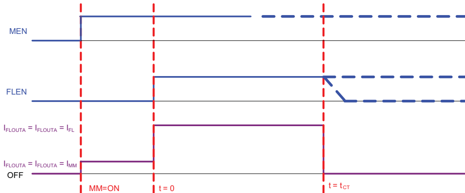
Figure 4: Diagram of Movie Mode Followed by Flash Mode When Flash Event is Terminated Before Flash Timer T_{FLASH} < T_{CT}^{1,2} .
