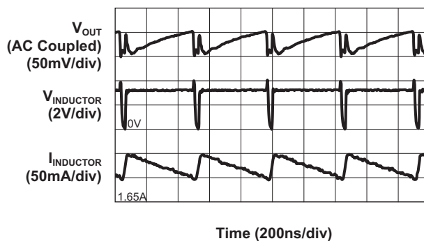
Flash Mode Output Ripple (I_{\text{FLOUT}} = 1.5\text{A}; V_{\text{IN}} = 4\text{V}; L = 1\mu\text{H})
