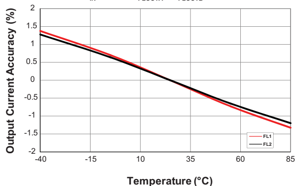
Movie Mode Current Accuracy vs. Temperature (V_{IN} = 3.6V; I_{FLOUTA} = I_{FLOUTB} = 50mA)
