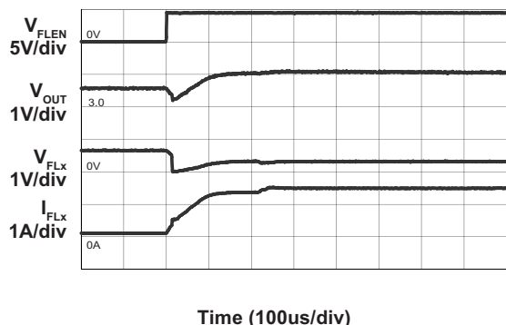
Movie Mode to Flash Turn On Characteristic (I_{\text{FLOUTA}} = I_{\text{FLOUTB}} = 50\text{mA to } 750\text{mA}; C_{\text{OUT}} = 1.0\mu\text{F}; V_{\text{IN}} = 3.6\text{V}; L = 1\mu\text{H})
