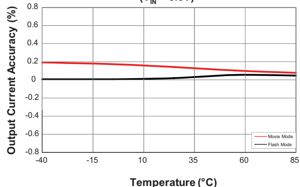
Flash and Movie Modes Current Matching vs. Temperature (V_{IN} = 3.6V)
