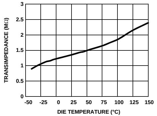
FIGURE 46. TRANSIMPEDANCE vs TEMPERATURE
