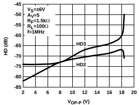
FIGURE 30. DIFFERENTIAL HARMONIC DISTORTION vs DIFFERENTIAL OUTPUT VOLTAGE (1/2 POWER MODE)
