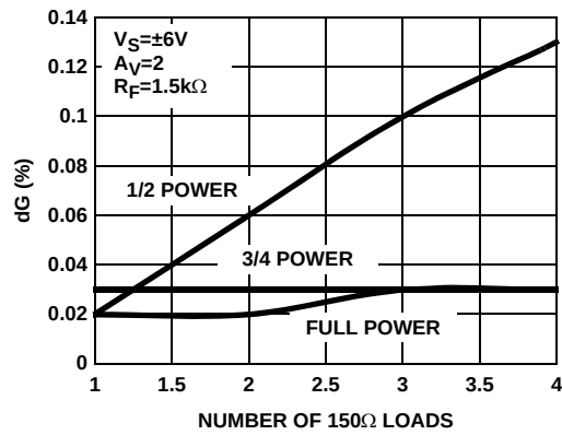
FIGURE 37. DIFFERENTIAL GAIN
