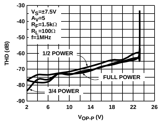
FIGURE 36. DIFFERENTIAL TOTAL HARMONIC DISTORTION vs DIFFERENTIAL OUTPUT VOLTAGE
