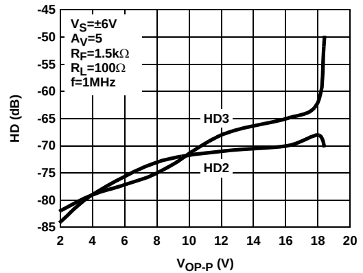
FIGURE 28. DIFFERENTIAL HARMONIC DISTORTION vs DIFFERENTIAL OUTPUT VOLTAGE (3/4 POWER MODE)
