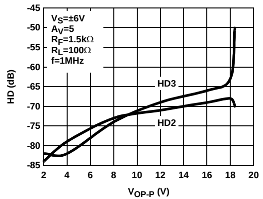
FIGURE 26. DIFFERENTIAL HARMONIC DISTORTION vs DIFFERENTIAL OUTPUT VOLTAGE (FULL POWER MODE)
