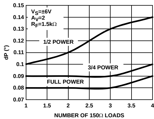
FIGURE 39. DIFFERENTIAL PHASE
