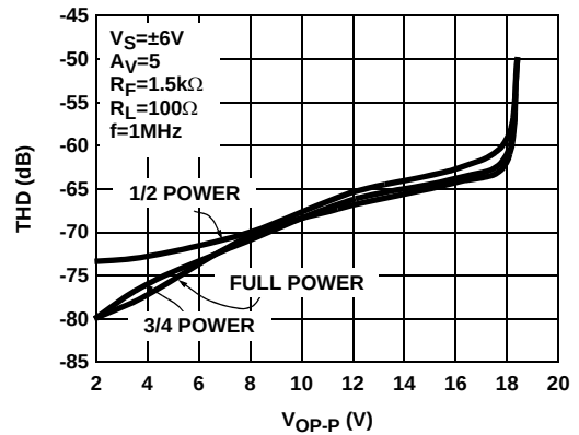
FIGURE 34. DIFFERENTIAL TOTAL HARMONIC DISTORTION vs DIFFERENTIAL OUTPUT VOLTAGE
