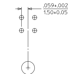
PCB LAYOUT: COMPONENT SIDE 4 CIRCUIT ONLY
