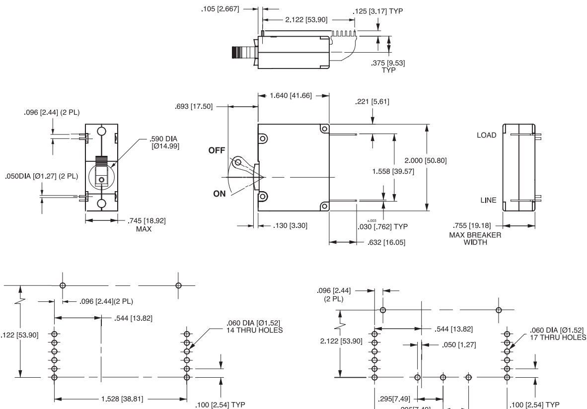
P.C. FOOT PRINT WITH AUX. SWITCH
