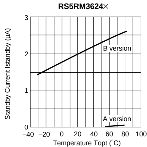
14) Standby Current vs. Temperature
