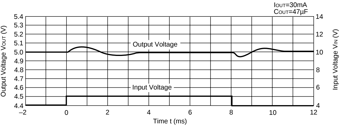
RS5RM5045A
