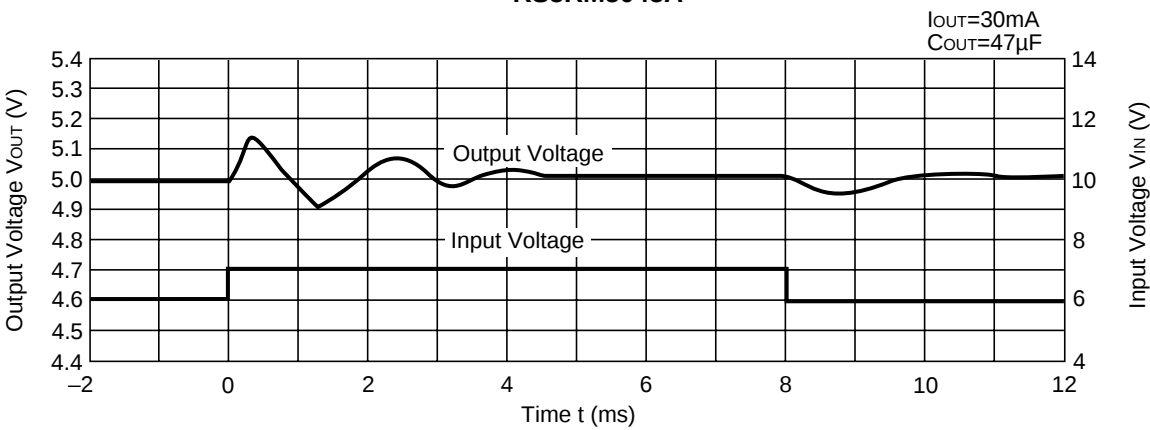
RS5RM5045A
