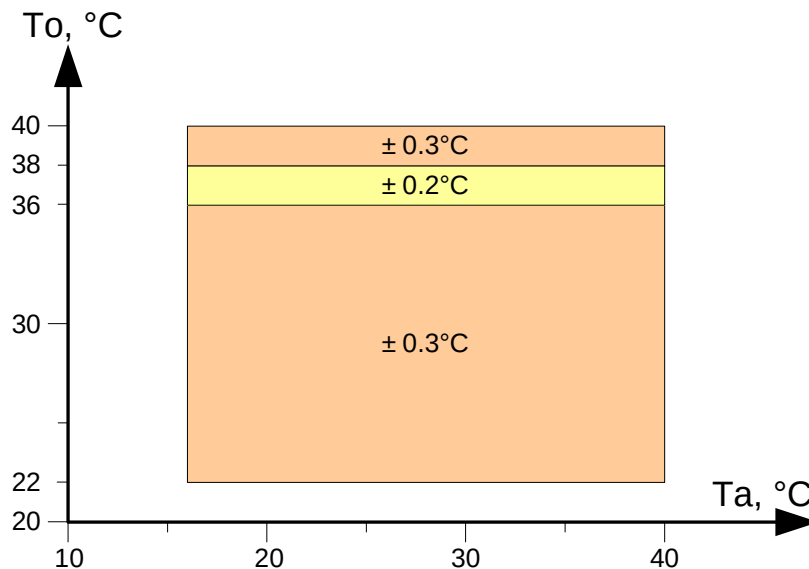
Figure 23: Accuracy of MLX90614DAA ( T_a , T_o ) for medical applications. Accuracy of the MLX90614DCC, DCH and DCI for V_{DD} = 3\text{V} (see paragraph 10.1.3)
