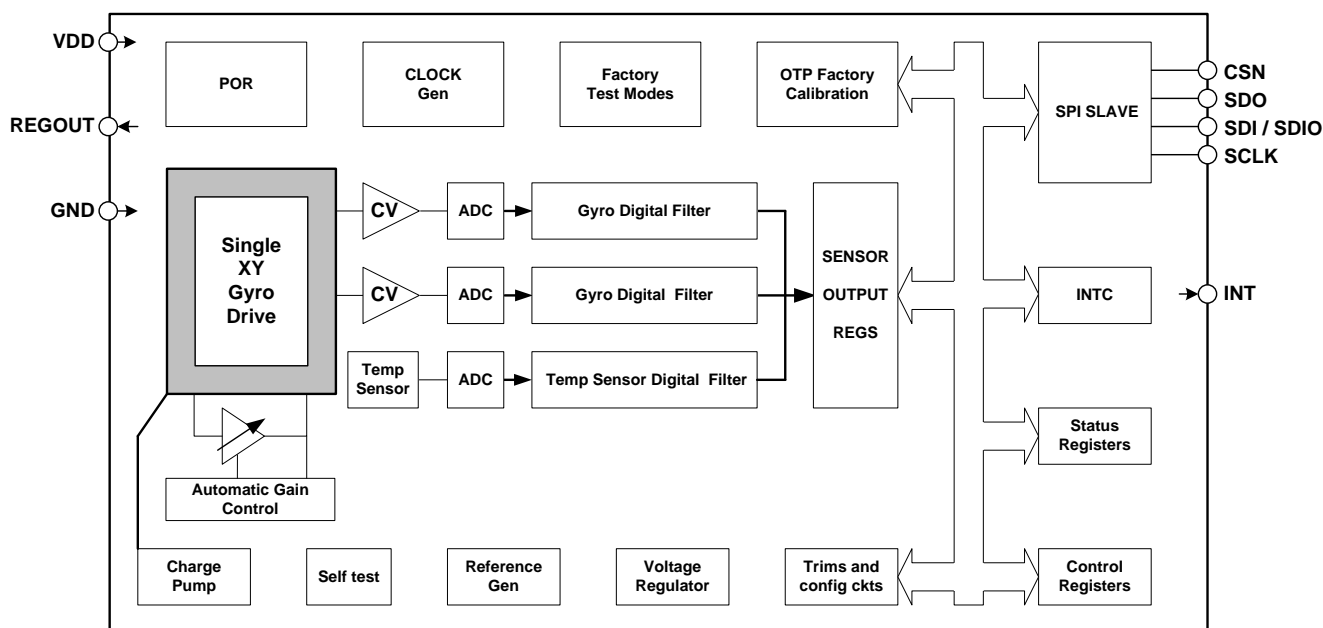
Figure 4. Block Diagram
