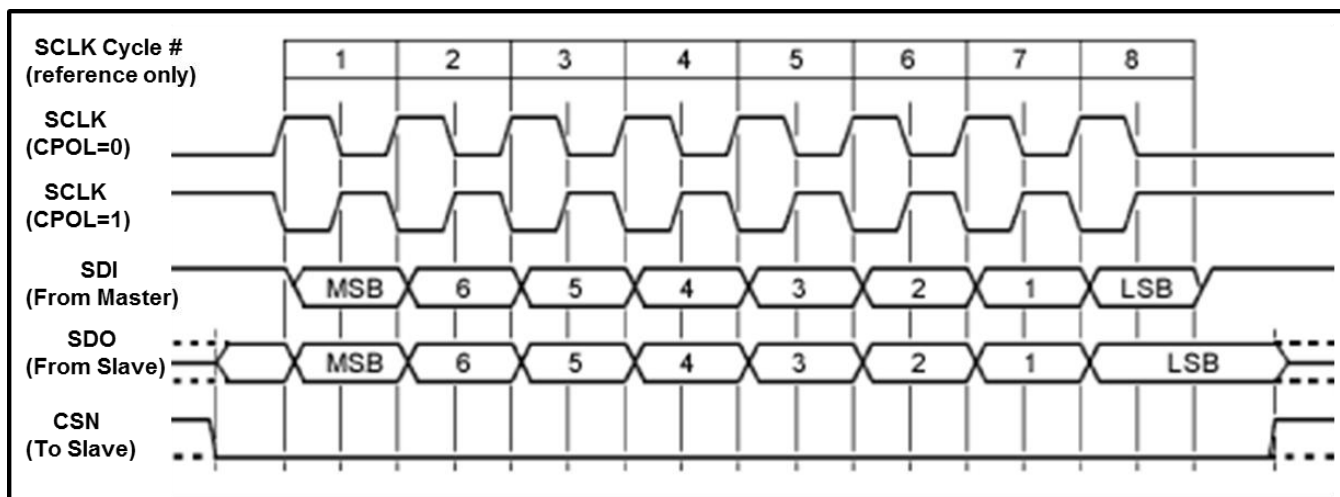
Figure 2b. 3-Wire interface timing with CPHA = 1 and CPOL = 0/1 3-wire Interface Clocks Data into the Slave on the Clock's Rising Edge and Data Out of the Slave on the Clock's Falling Edge
