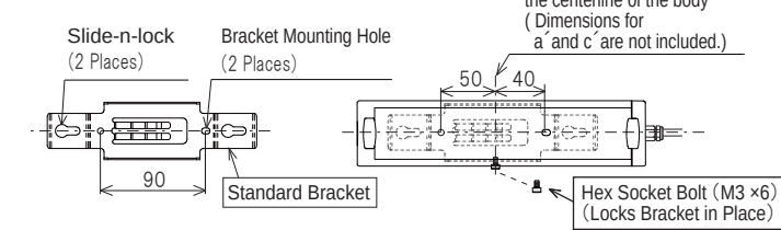
Figure 1. AG Type Installation -1
