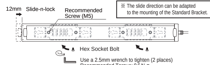
Figure 7. AG Type Slide Installation -2
