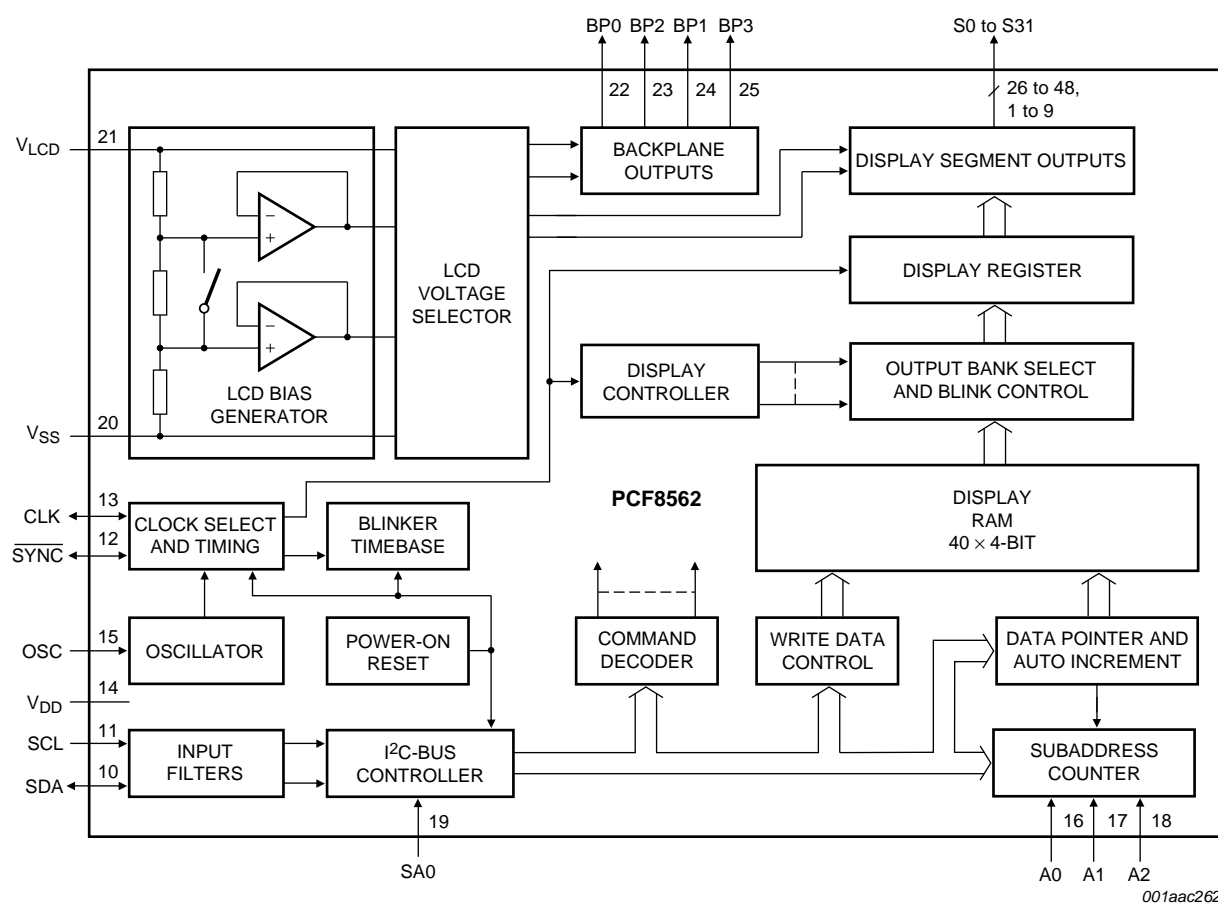
Fig 1. Block diagram of PCF8562
