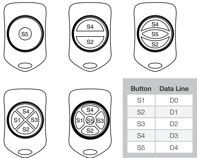
Figure 6: OTX-***-HH-KF#-MS Button Assignments
