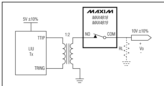
Figure 1. Fault Protection
