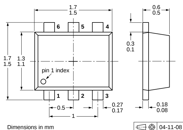
Fig 17. Package outline PEMD2 (SOT666)
