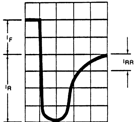
REVERSE RECOVERY WAVE FORM
