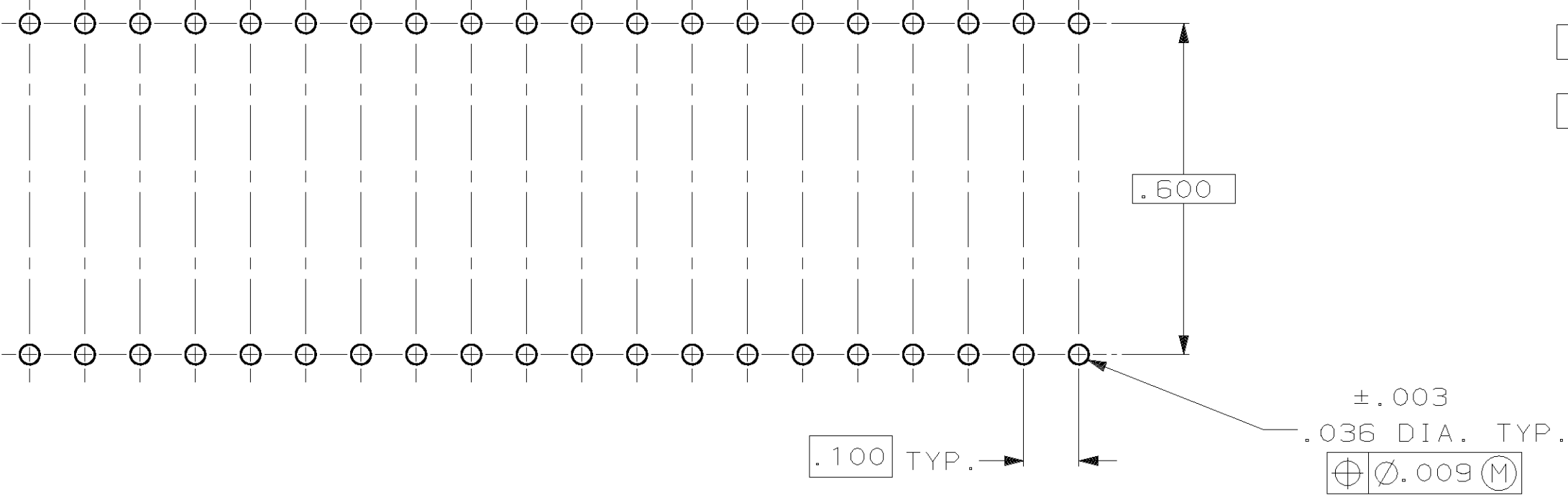
RECOMMENDED MOUNTING HOLE PATTERN SCALE 4:1
