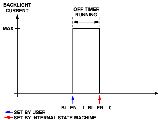
Figure 35. Off Timer
