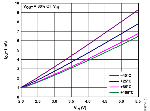
Figure 15. Typical Soft Start Current, I_{SS}
