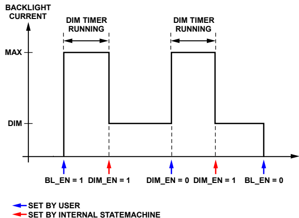
Figure 34. Dim Timer
