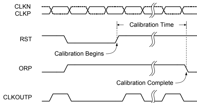
FIGURE 21. CALIBRATION TIMING
