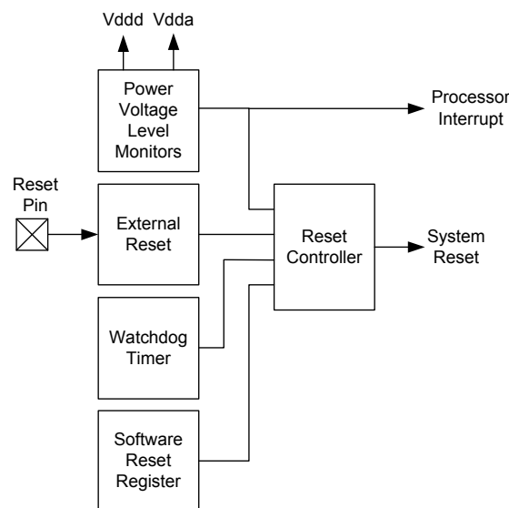
Figure 6-7. Resets
