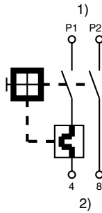
1-pole thermal protected, non illuminated
