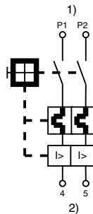
2-pole thermal and magnetic protected, non illuminated
