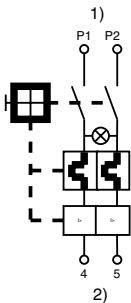
2-pole thermal and magnetic protected, illuminated
