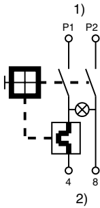
1-pole thermal protected, illuminated
