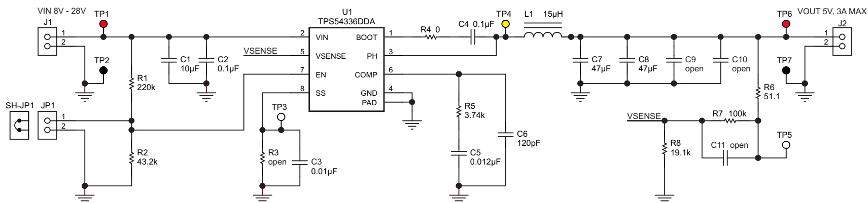
Figure 18. TPS54336EVM-556 Schematic
