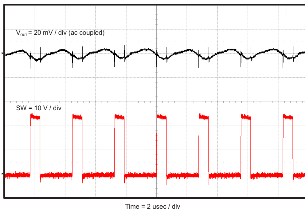
Figure 7. TPS54336EVM-556 Output Ripple, I_{OUT} = 3 A
