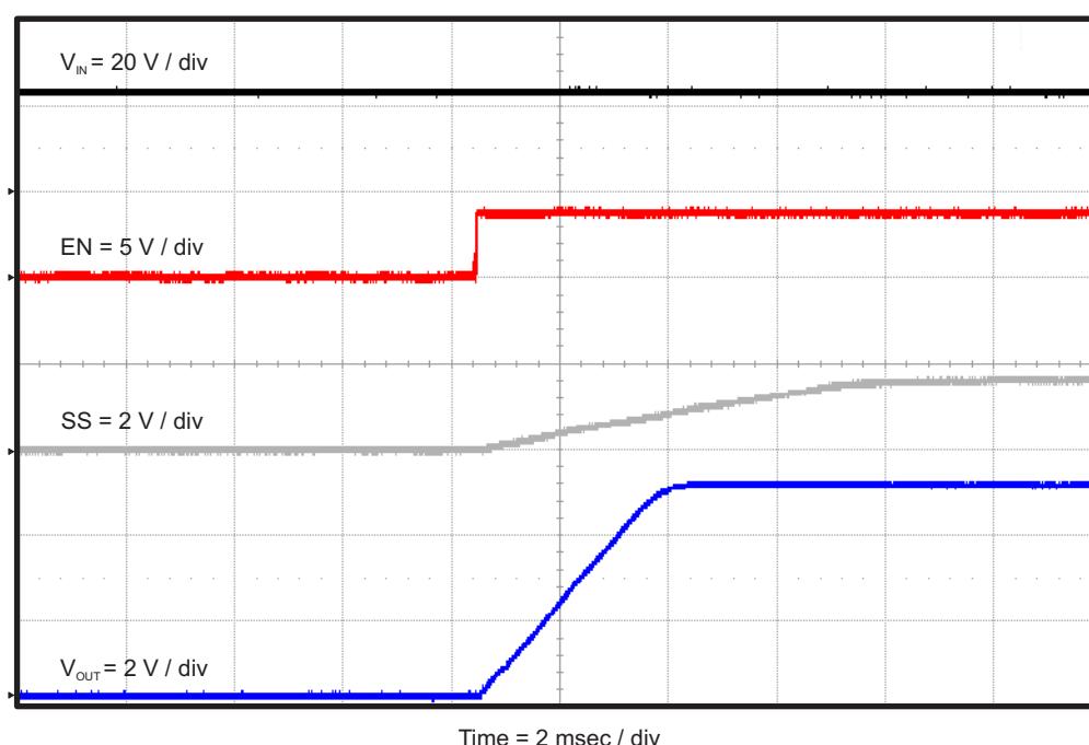
Figure 12. TPS54336EVM-556 Start-up Relative to Enable
