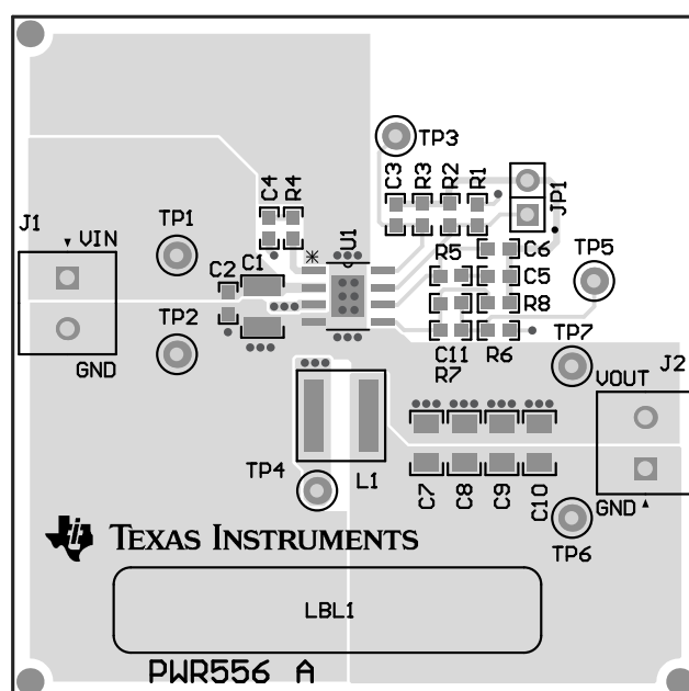
Figure 15. TPS54336EVM-556 Top-Side Assembly
