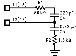
FIGURE 5. Loudness Control Circuit
