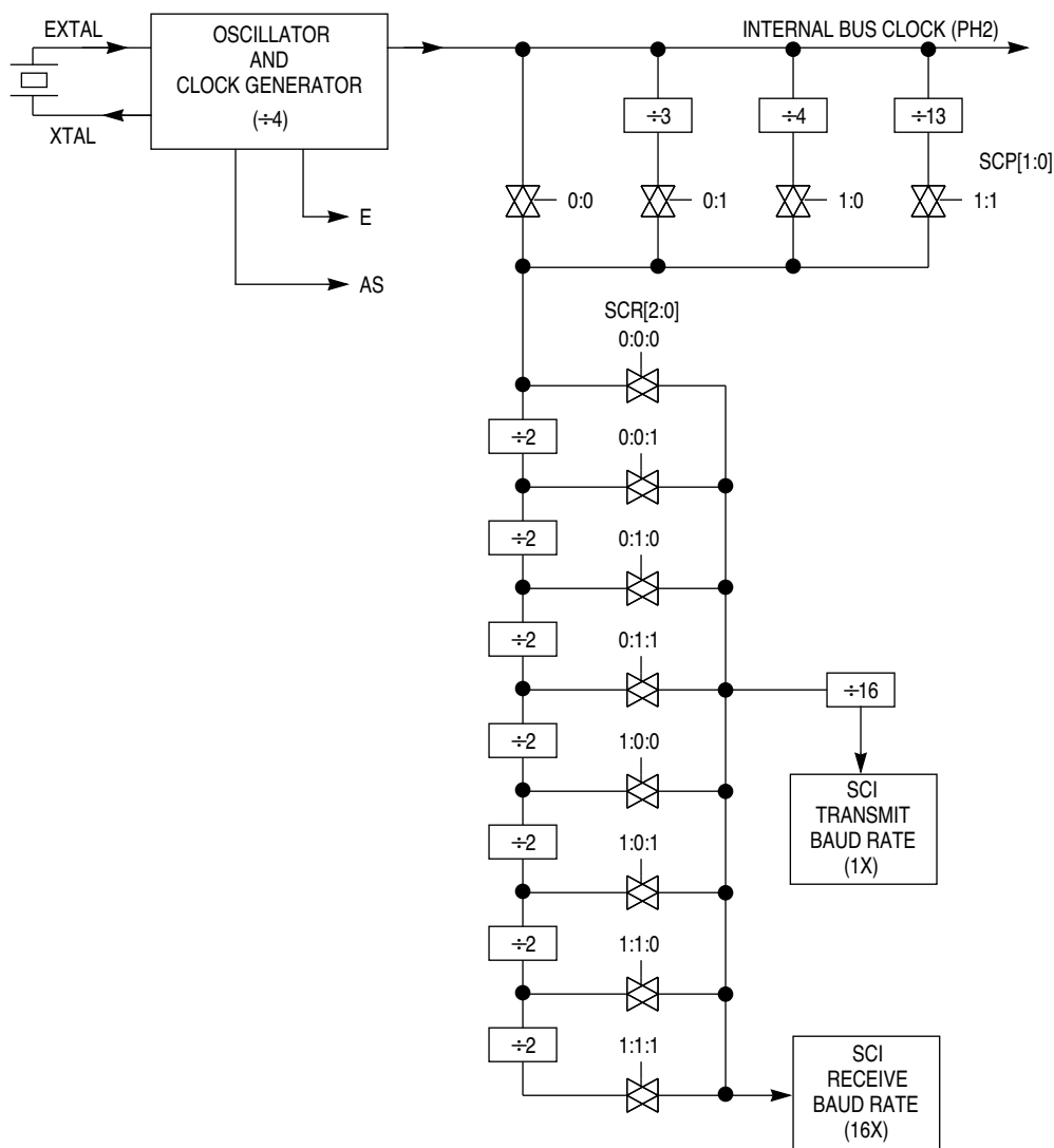
Figure 8 SCI Baud Rate Diagram
