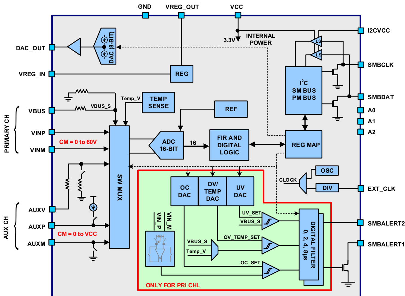
FIGURE 2. BLOCK DIAGRAM
