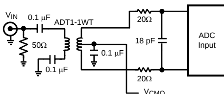
Figure 32. Low Input Frequency Transformer Drive Circuit
