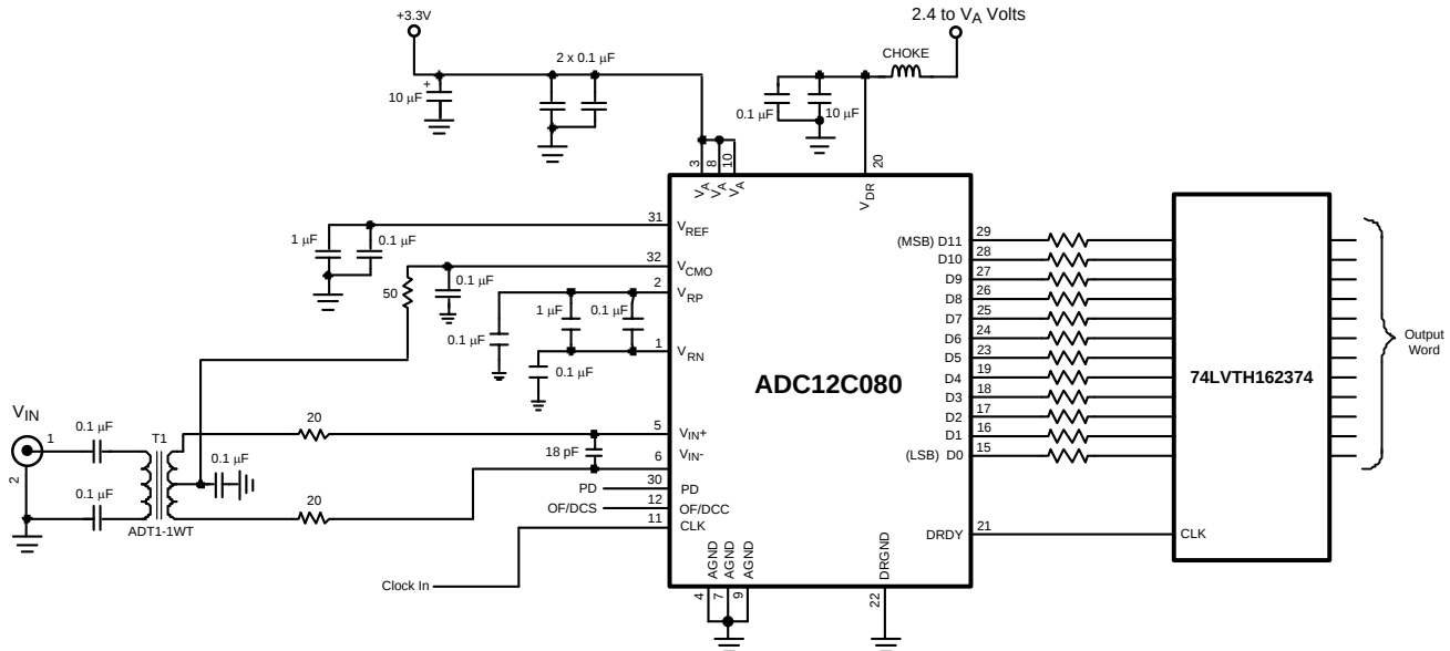
Figure 34. Application Circuit
