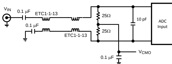
Figure 33. High Input Frequency Transformer Drive Circuit
