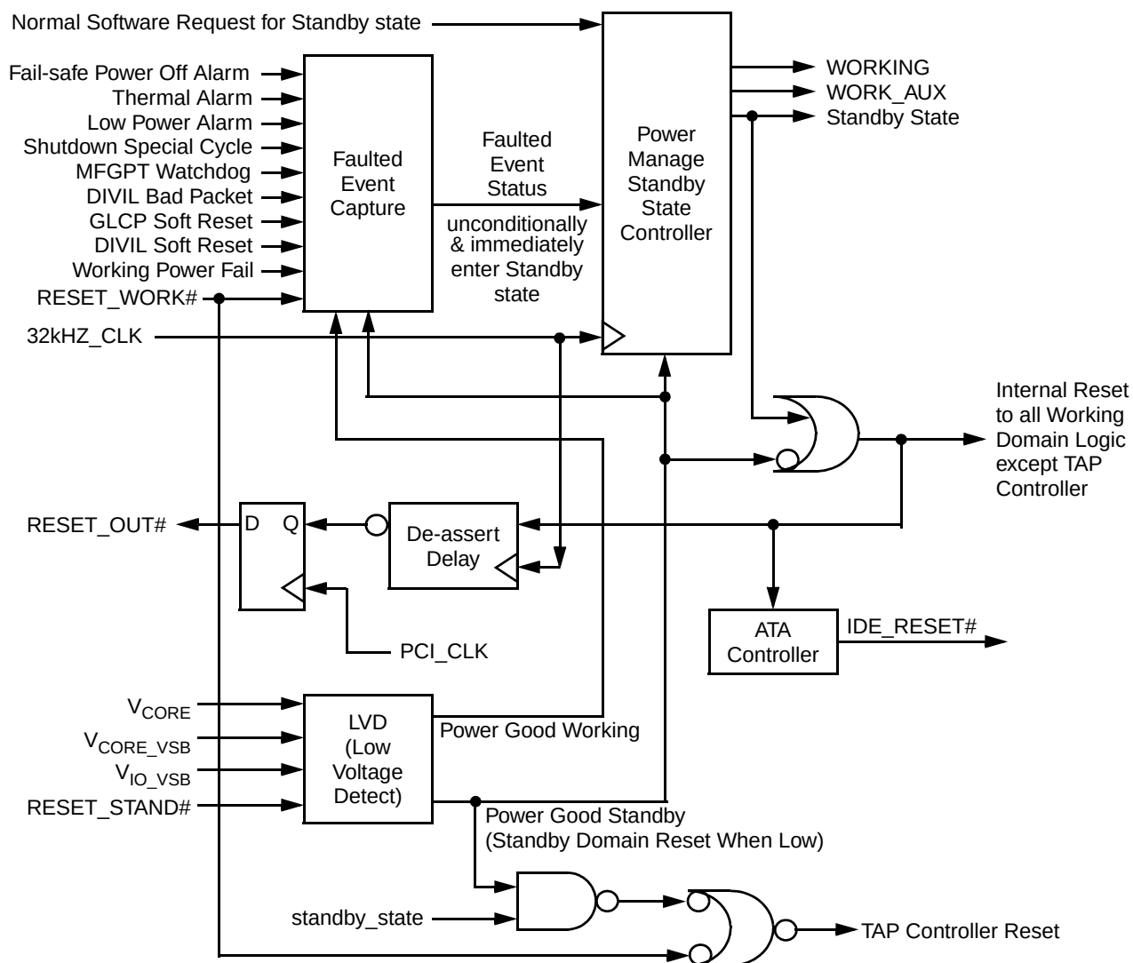
Figure 4-6. Reset Logic
