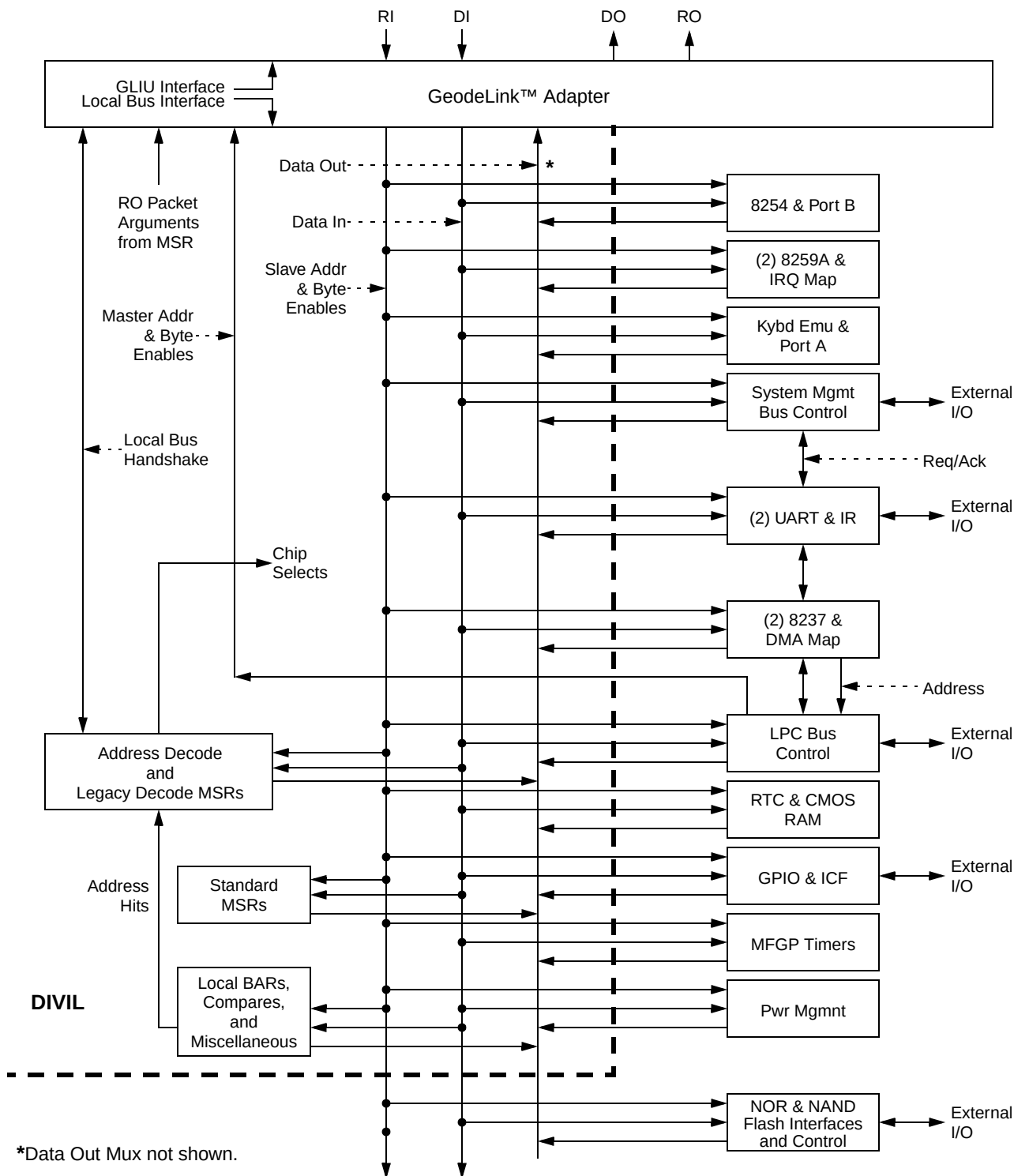
Figure 5-10. Diverse Logic Block Diagram
