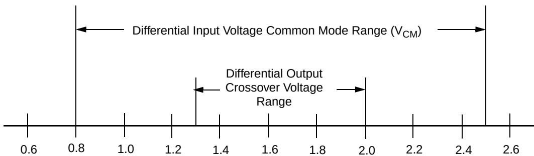
Figure 7-10. USB Differential Input Sensitivity Range
