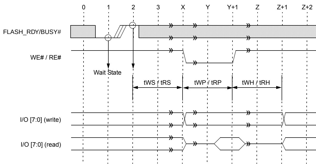
Figure 5-61. NAND Data Timing with Wait States
