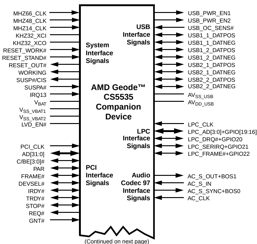
Figure 3-1. Typical Signal Groups
