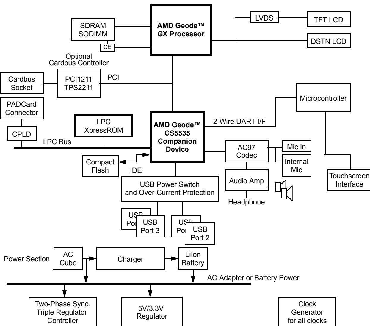
Figure 2-1. Typical WebPAD™ System Block Diagram
