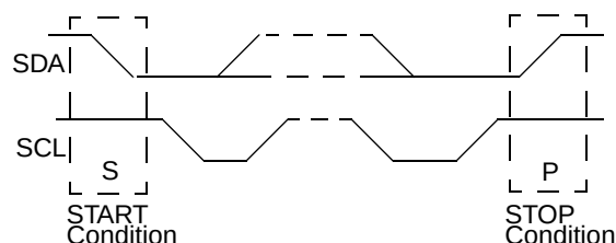
Figure 5-25. SMB START and STOP Conditions
