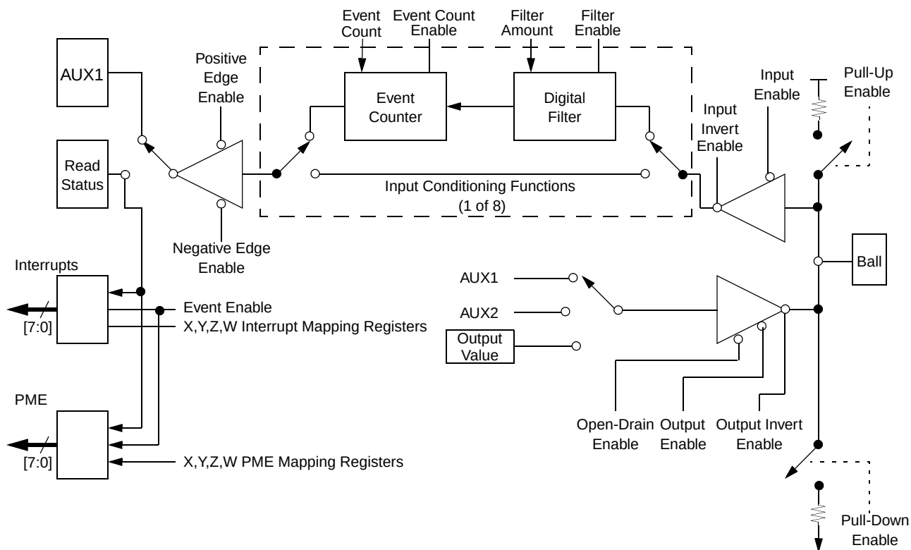
Figure 5-49. GPIO Configuration
