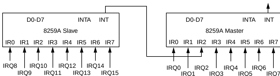
Figure 5-19. Cascading 8259As for LPIC
