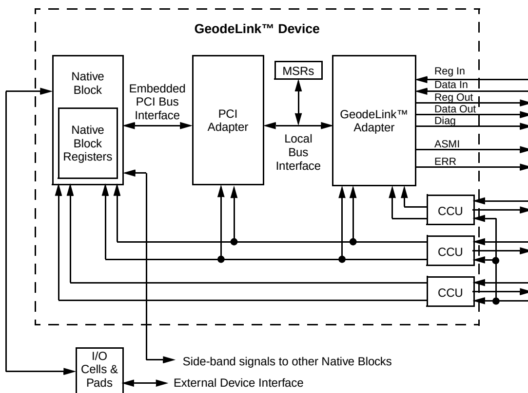
Figure 4-5. GeodeLink™ Device With Embedded PCI Bus
