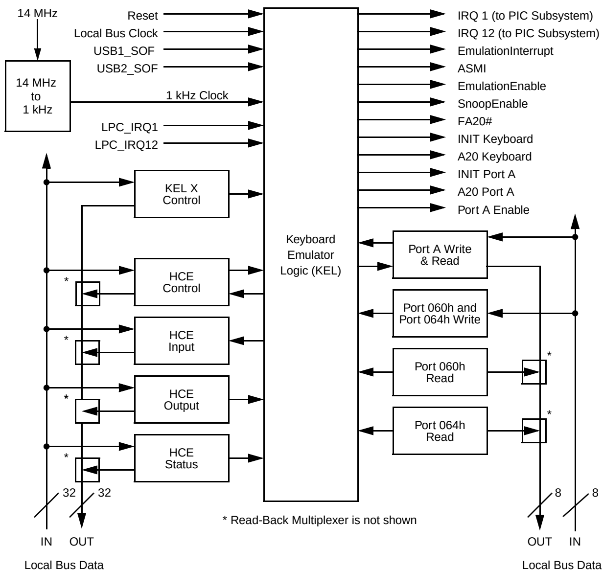
Figure 5-22. KEL Block Diagram
