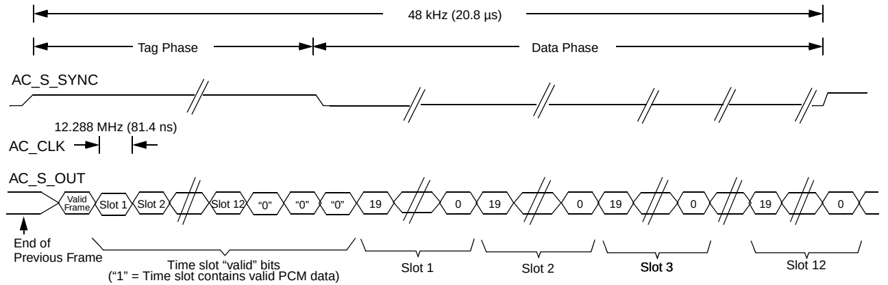
Figure 5-5. AC Link Output Frame
