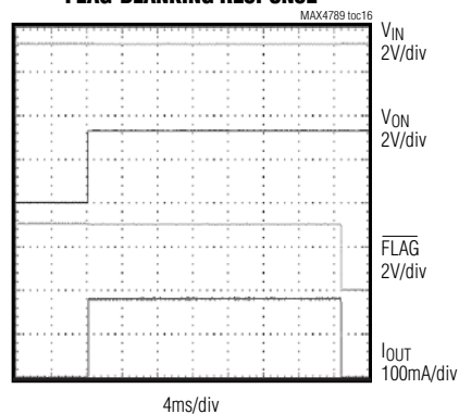
FLAG-BLANKING RESPONSE
