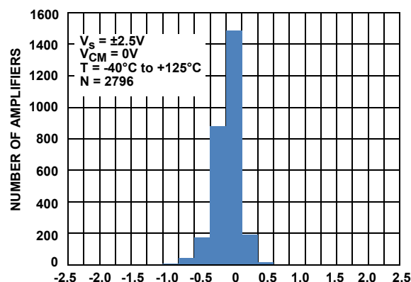
FIGURE 2. V_{OS} HISTOGRAM V_S = 5\text{V}
