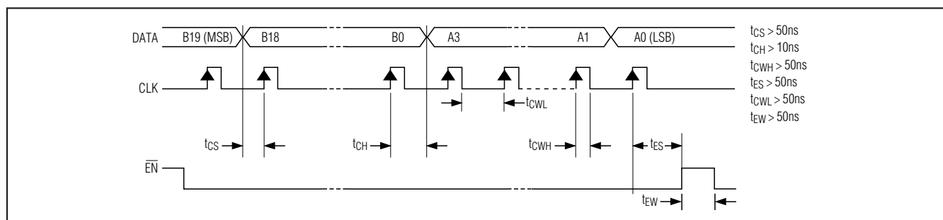
Figure 1. 3-Wire Interface Timing Diagram
