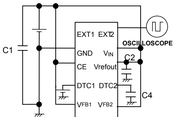
● Test Circuit 13
