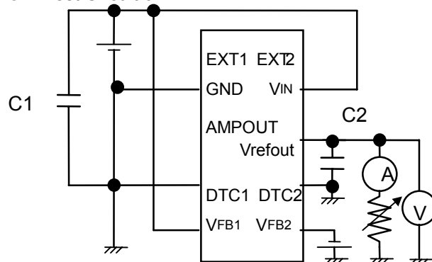
● Test Circuit 8
