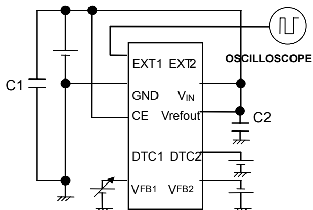
● Test Circuit 14
