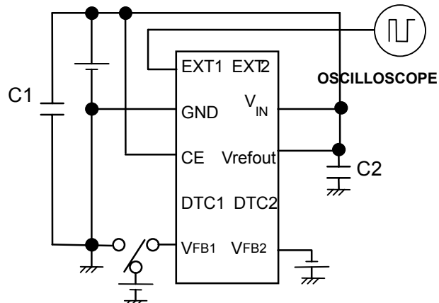
● Test Circuit 16
