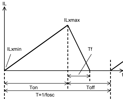
Discontinuous Mode
