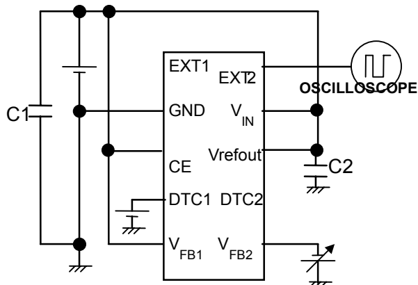
● Test Circuit 15
