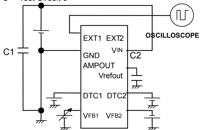
● Test Circuit 5
