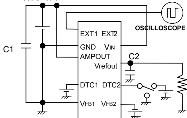
● Test Circuit 7
