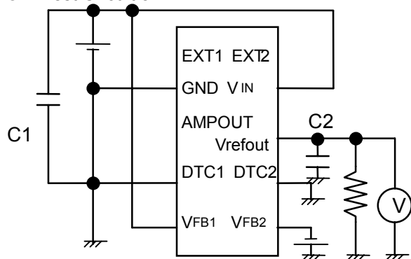
● Test Circuit 7
