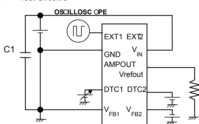
● Test Circuit 8
