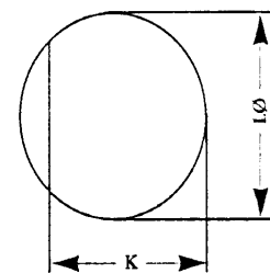
Recommended Panel Cutout (For Single Hole Mounting)
