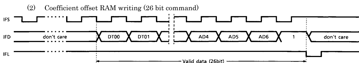
Figure 3 Example \mu -COM I/F
