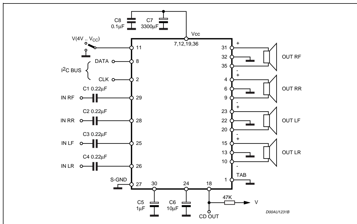
Figure 4. Application Circuit
