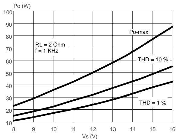
Figure 7. Output Power vs. Supply Voltage (2 \Omega )
