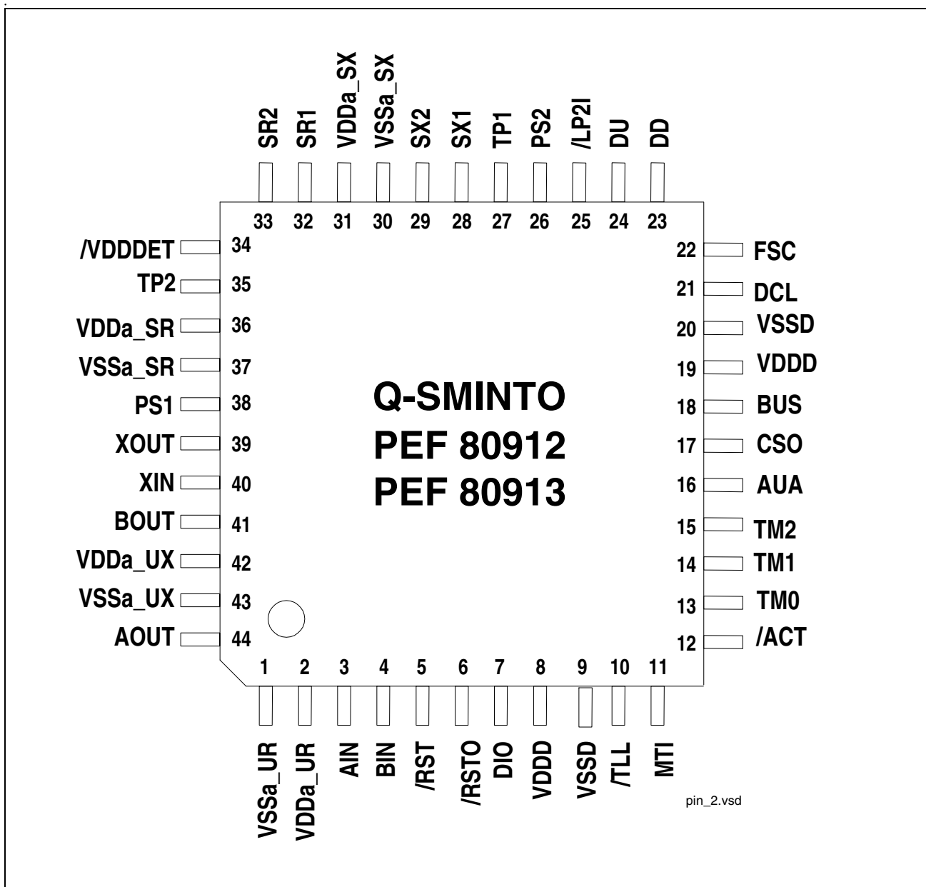
Figure 1 Pin Configuration
