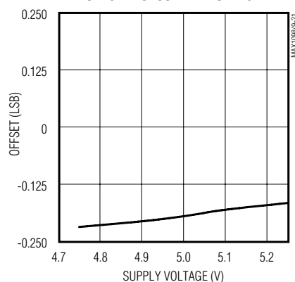
MAX1098 OFFSET vs. SUPPLY VOLTAGE
