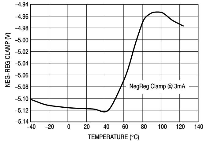
Figure 8. NegReg Clamp @ 3mA versus Temperature
