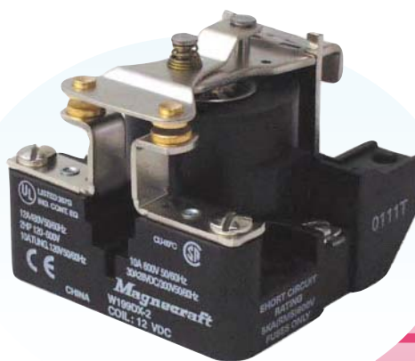
199 SPST-NO-DM 30 AMPS, 2 Hp
