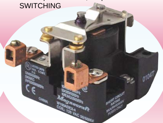
199DE SPST-NO-DM WITH BOX TERMINALS. 50 AMPS, 2 Hp
