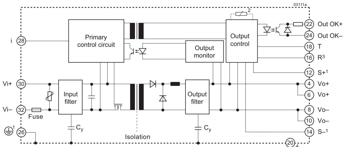
Fig. 6 Block diagram of a single-output converter 1 Leading pins 2 Potentiometer for option P 3 Do not connect for models xQ1101 or with option P 4 Do not connect
