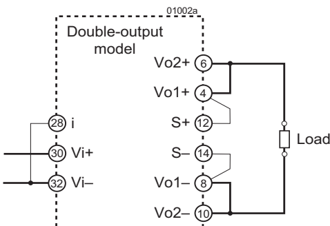
Fig. 2 Parallel-output configuration
