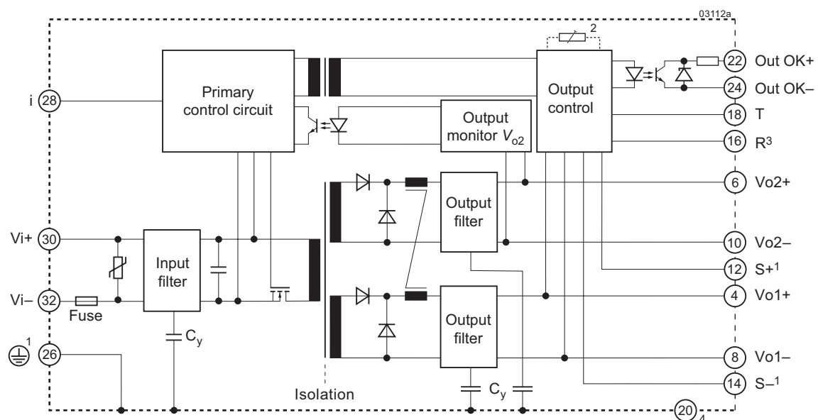
Fig. 7 Block diagram of a double-output converter 1 Leading pins 2 Potentiometer for option P 3 Do not connect for models with option P 4 Do not connect
