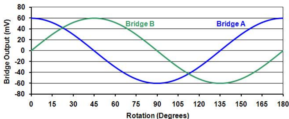
Figure 4. Typical Bridge Outputs vs Rotation Angle
