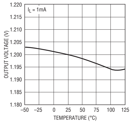
LT1761-1.2 Output Voltage
